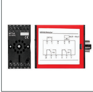
LOOP DETECTOR
