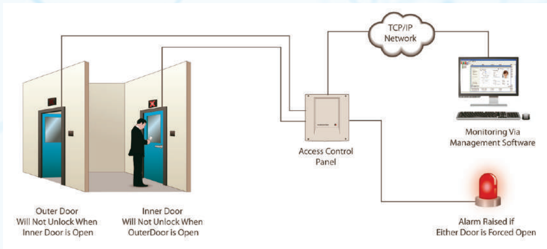
Door Interlock Access Control System
